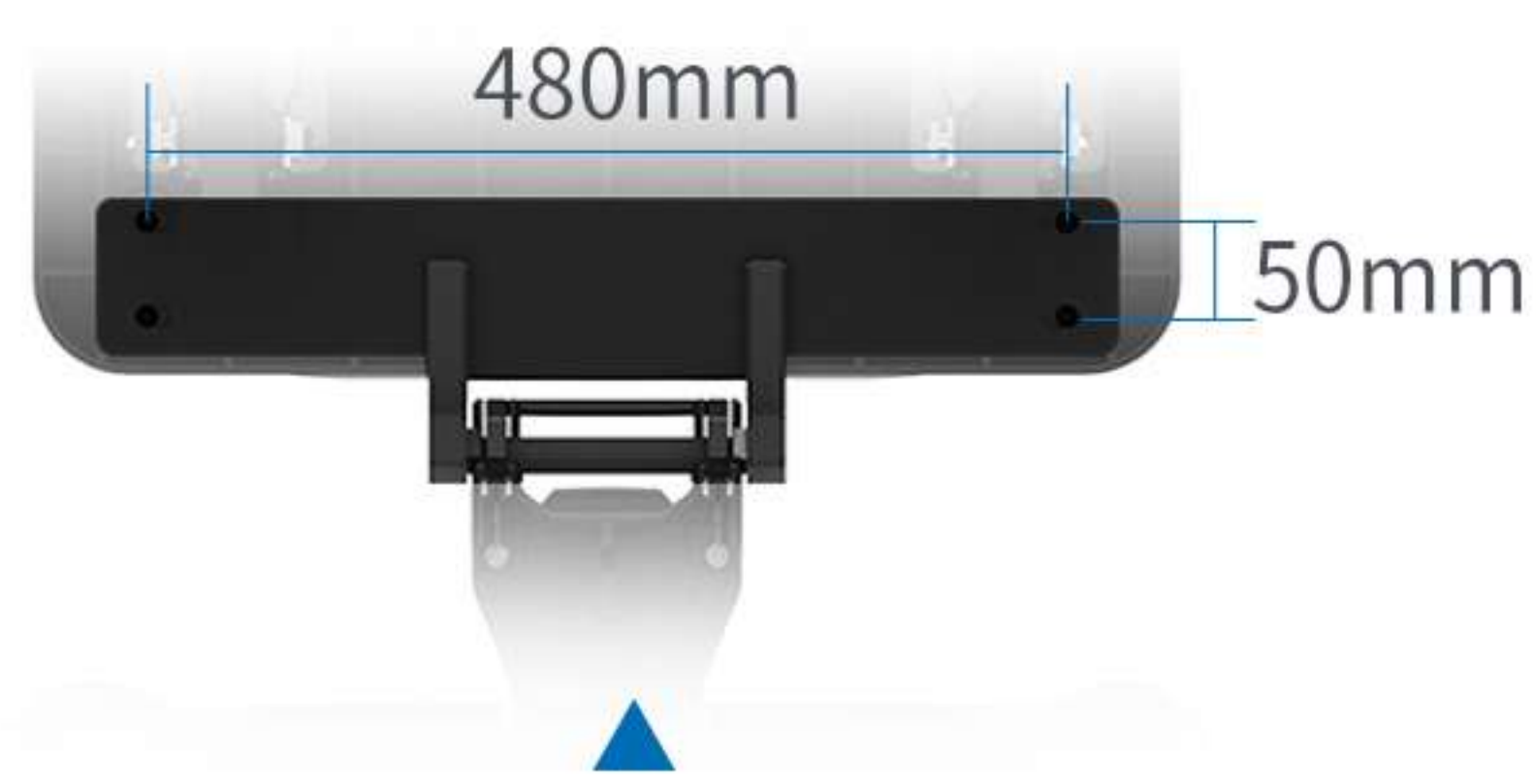
Cart Adaptive Mounting Hole Dimensions
